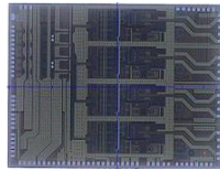
ms86040/ms87040 chipsets –for 200G SR4/400G SR8 application
